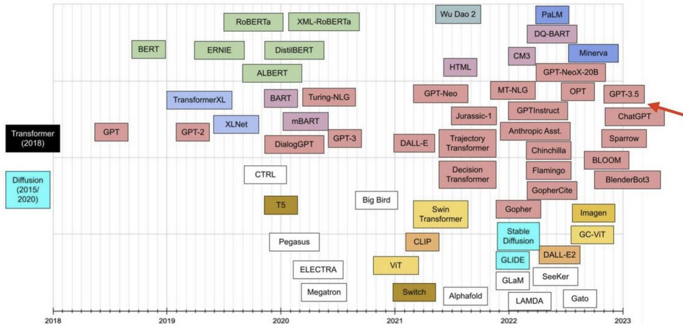
Figure 7: Transformer timeline. Colors describe Transformer family.
